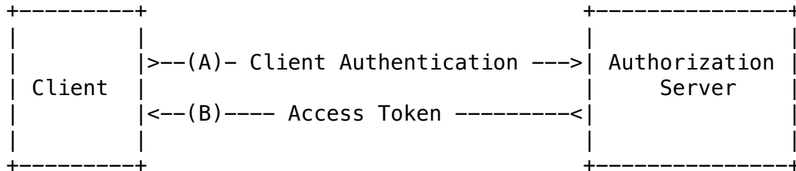
Figure 6: Client Credentials Flow
