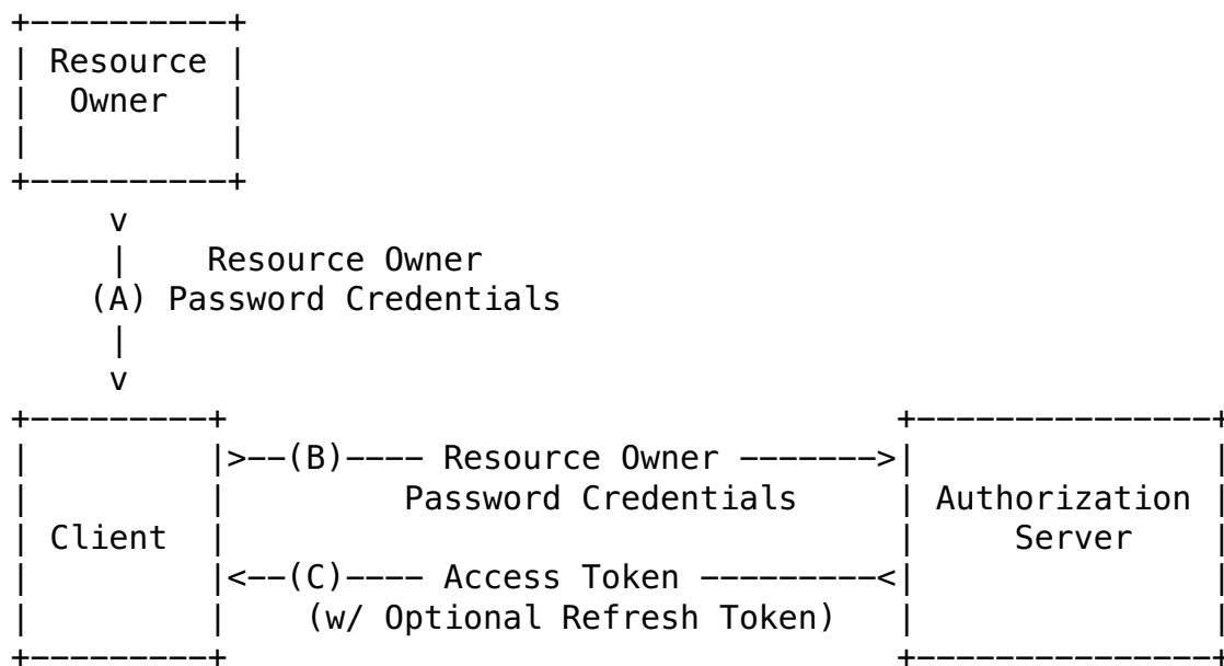
Figure 5: Resource Owner Password Credentials Flow
